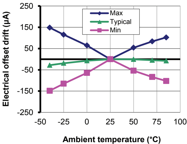
Figure 3: Electrical offset thermal drift
