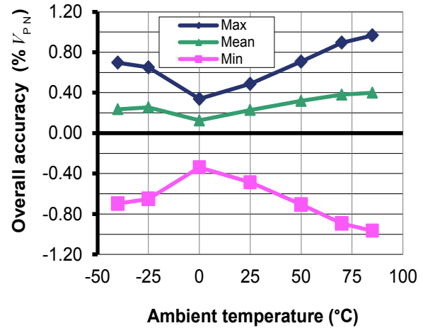
Figure 4: Overall accuracy in temperature
