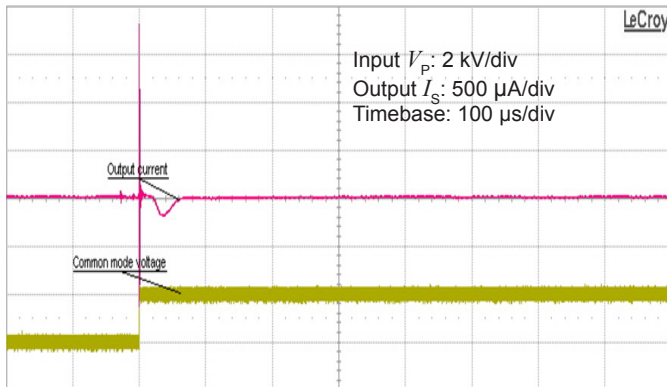
Figure 11: Typical common mode perturbation (2000 V step with 6 kV/µs R_M = 100 \Omega )
