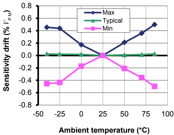
Figure 5: Sensitivity thermal drift
