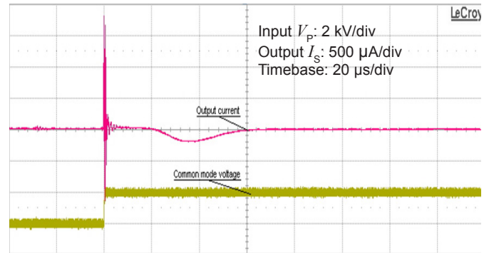
Figure 12: Detail of typical common mode perturbation (2000 V step with 6 kV/µs, R_M = 100 \Omega )
