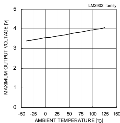
Fig. 77 Maximum Output Voltage - Ambient Temperature (VCC=5[V], RL=2[kΩ])
