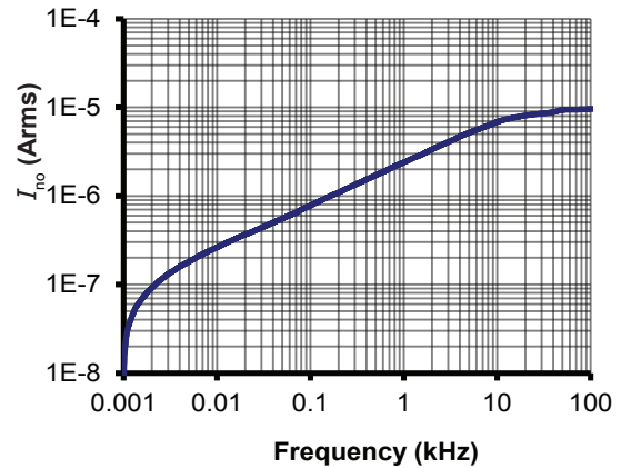
Figure 14: Typical total output rms current noise with R_M = 50 \Omega
