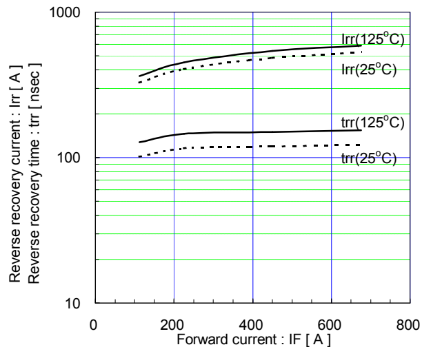
Reverse recovery characteristics (typ.) V_{CC}=600\text{V} , V_{GE}=\pm 15\text{V} , R_G=0.68\Omega
