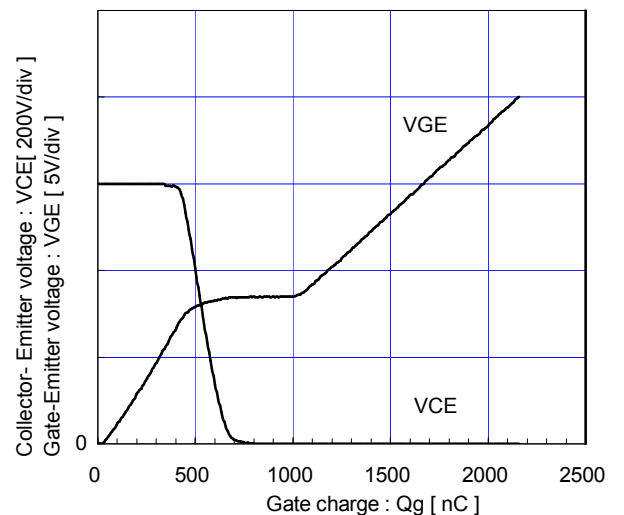
Dynamic Gate charge (typ.) Vcc=600V, Ic=450A, Tj=25°C
