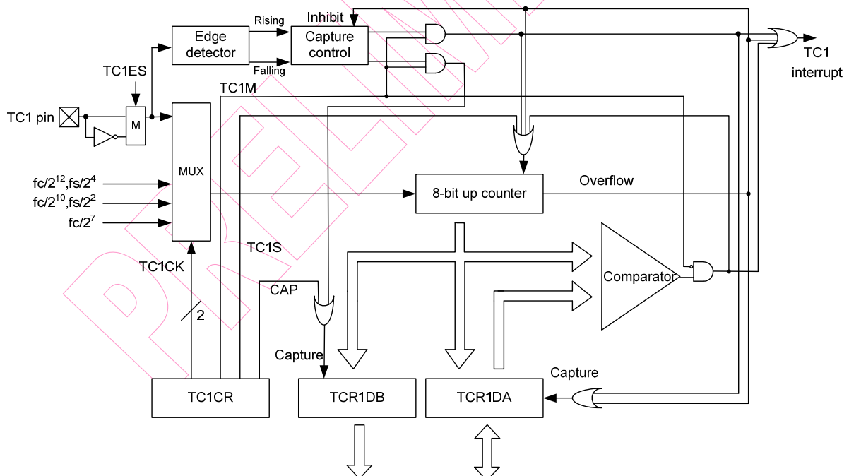
Fig.6 Configuration of Timer/Counter1
