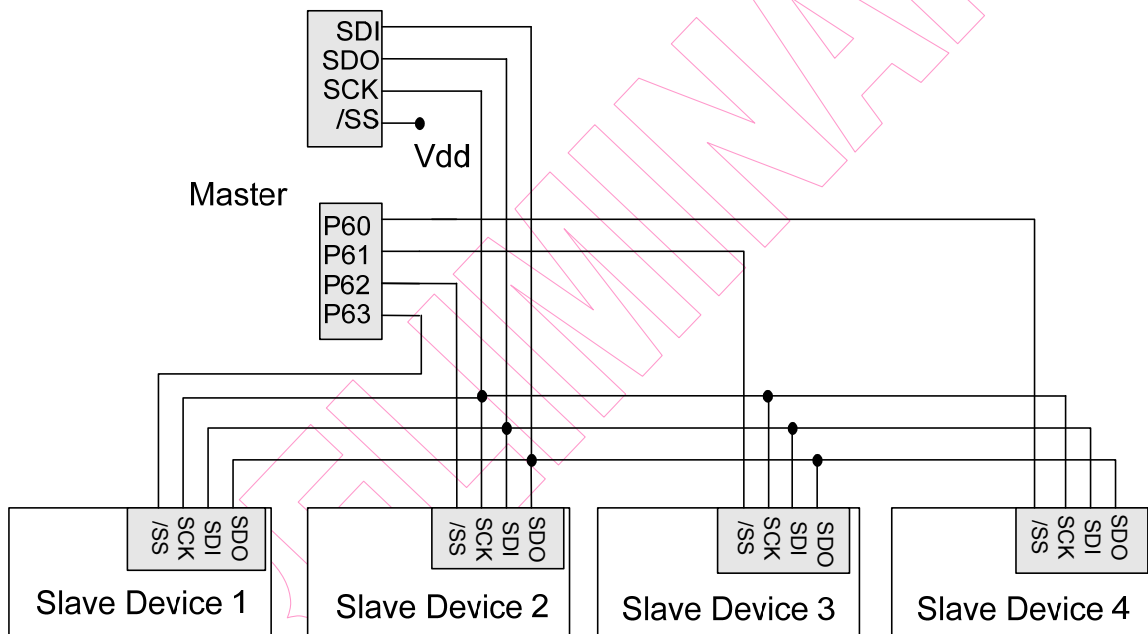
Fig. 21 The SPI Configuration of Single-Master and Multi-Slave
