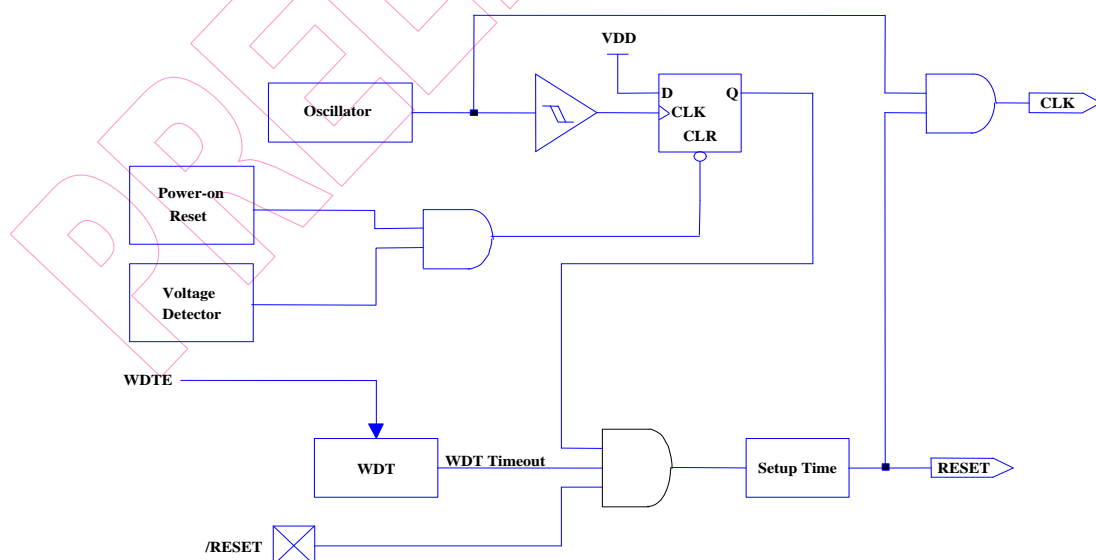
Fig. 30 Block Diagram of Controller Reset
