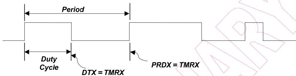
Fig. 29 The Output Timing of the PWM
