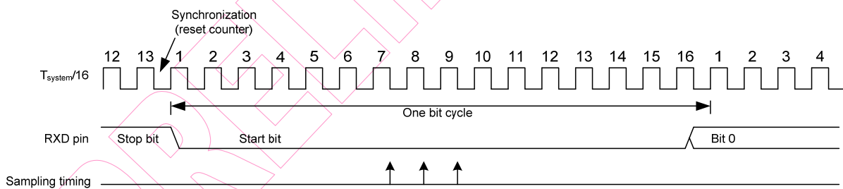
Fig. 19 UART timing
