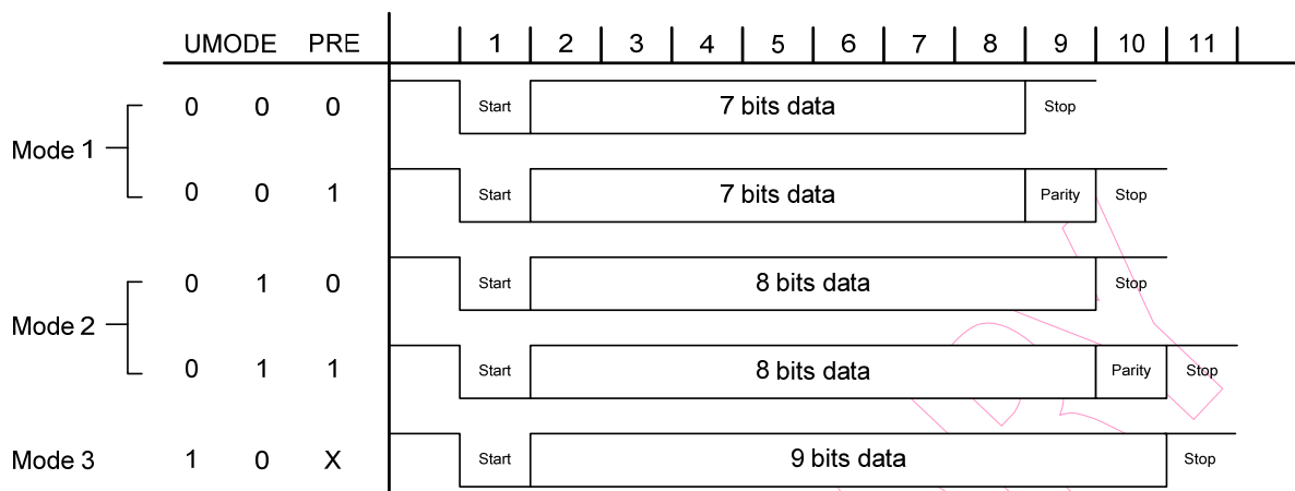
Fig. 18 UART Model
