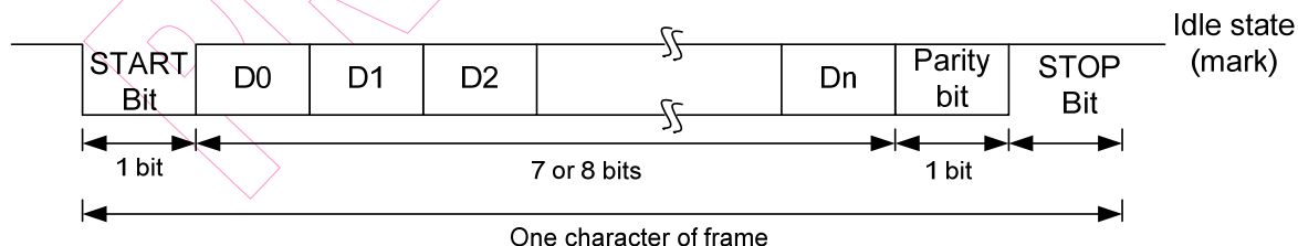
Fig. 17 Data Format in UART
