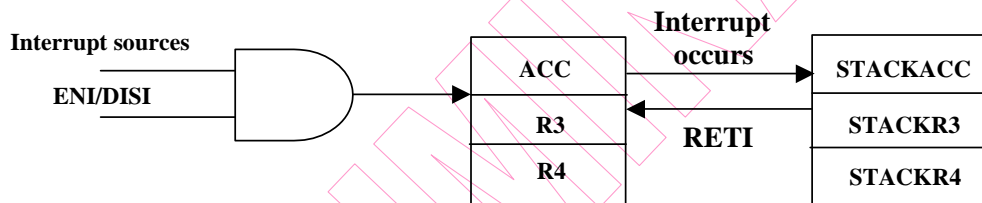
Fig. 32 Interrupt backup diagram
