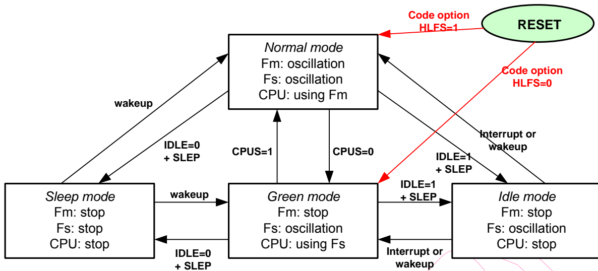
Fig. 5 CPU operation mode
