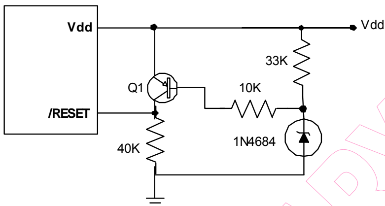
Fig. 38 Circuit 1 for the Residue Voltage Protection
