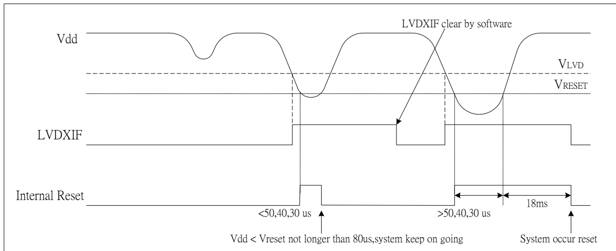
Fig. 33 LVD waveform situation
