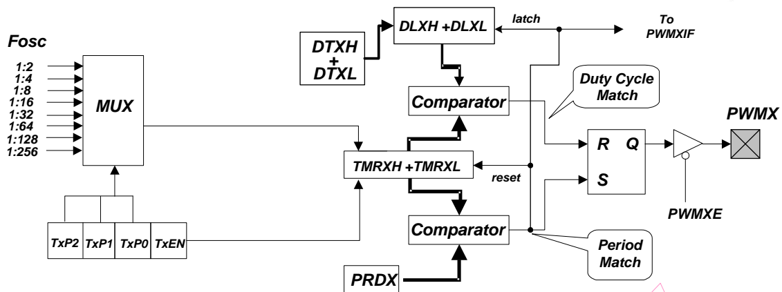
Fig. 28 The Functional Block Diagram of the Three PWMs
