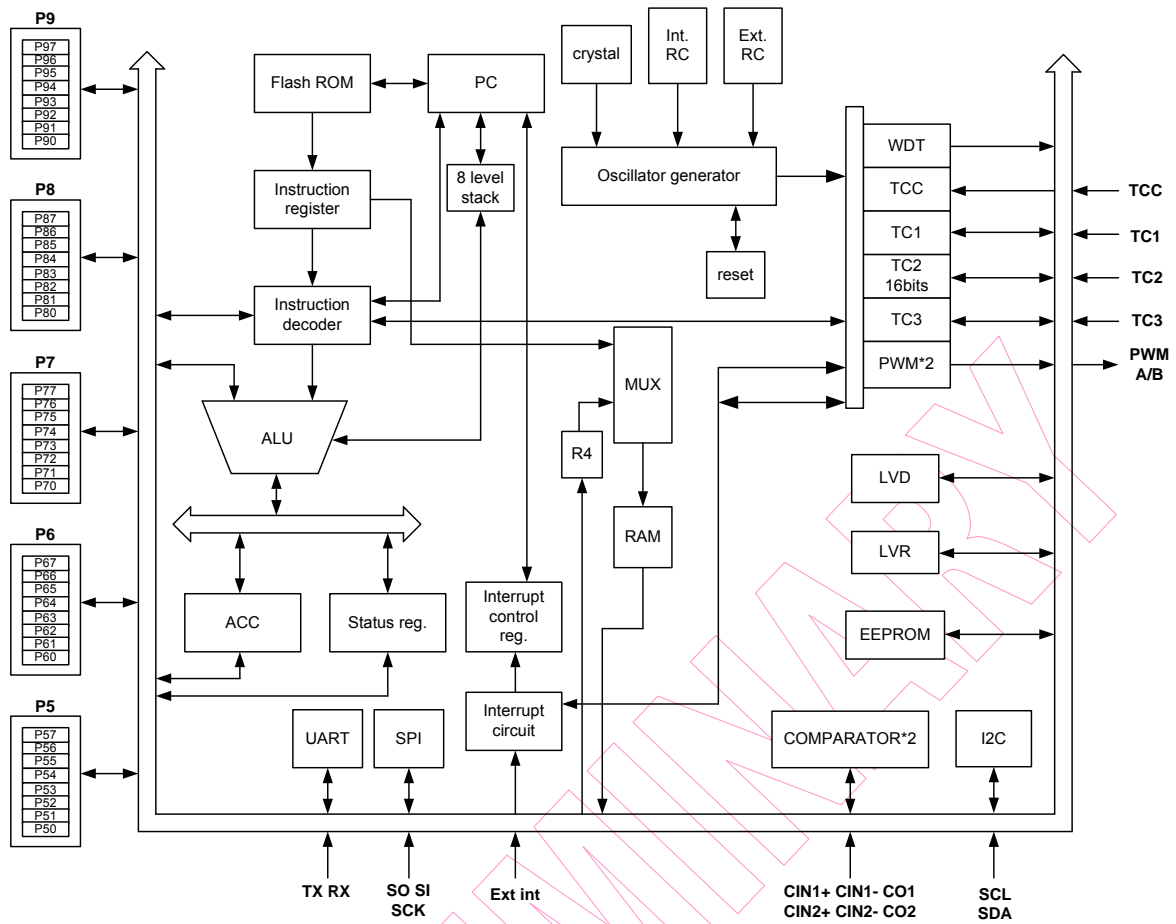
Fig. 2 Function Block Diagram
