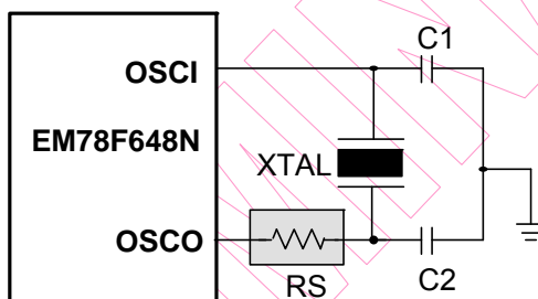
Fig. 35 Circuit for Crystal/Resonator
