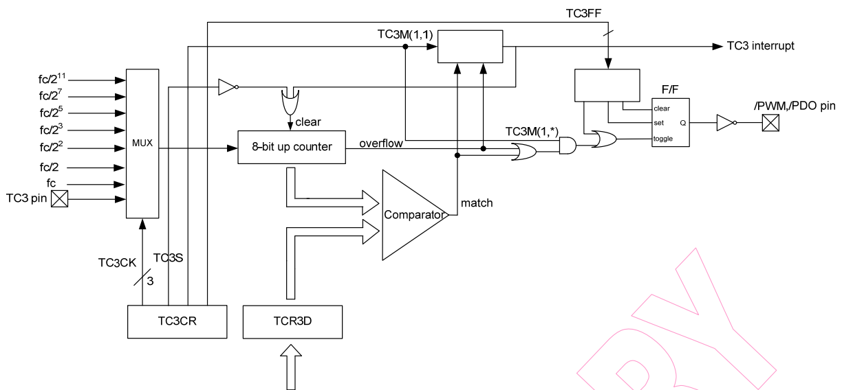
Fig. 12 Timer/Counter3 Configuration
