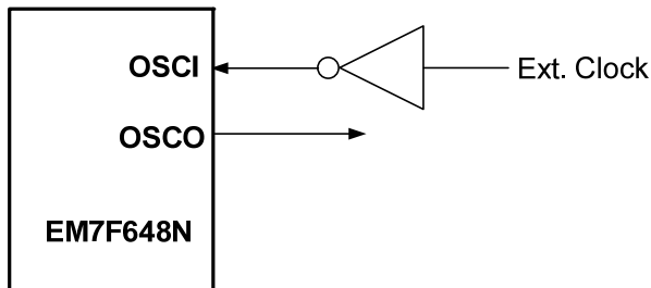
Fig. 34 Circuit for External Clock Input
