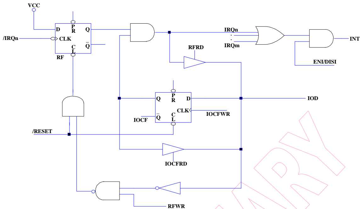
Fig. 31 Interrupt Input Circuit
