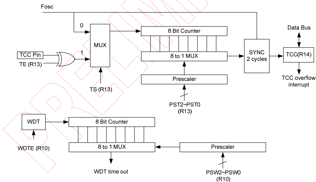
Fig. 15 Block Diagram of TCC and WDT
