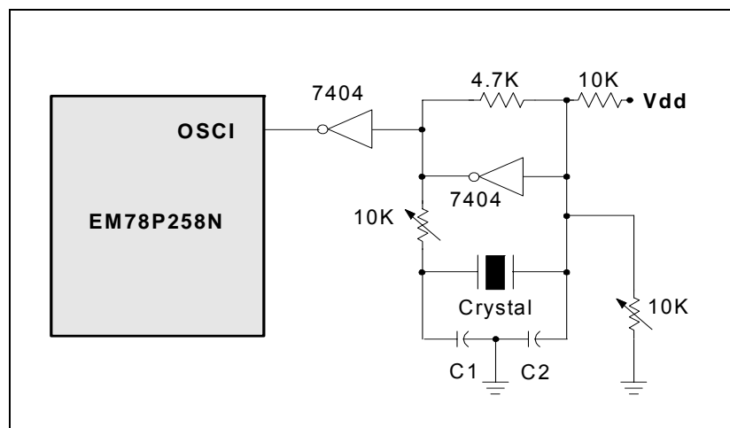
Fig 6-17 Parallel Mode Crystal/Resonator Circuit Diagram
