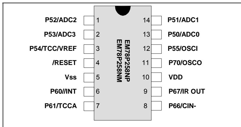
Fig 3-1 Pin Assignment – EM78P258NP/M
