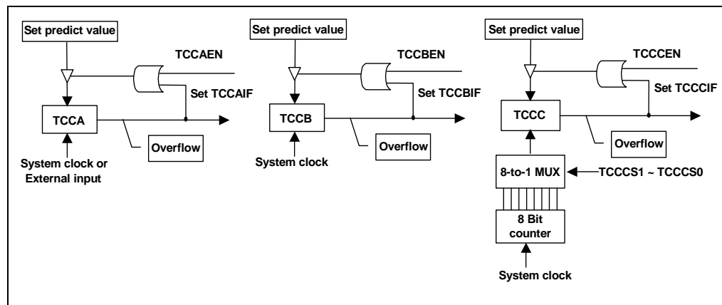
Fig 6-13 Timer Block Diagram
