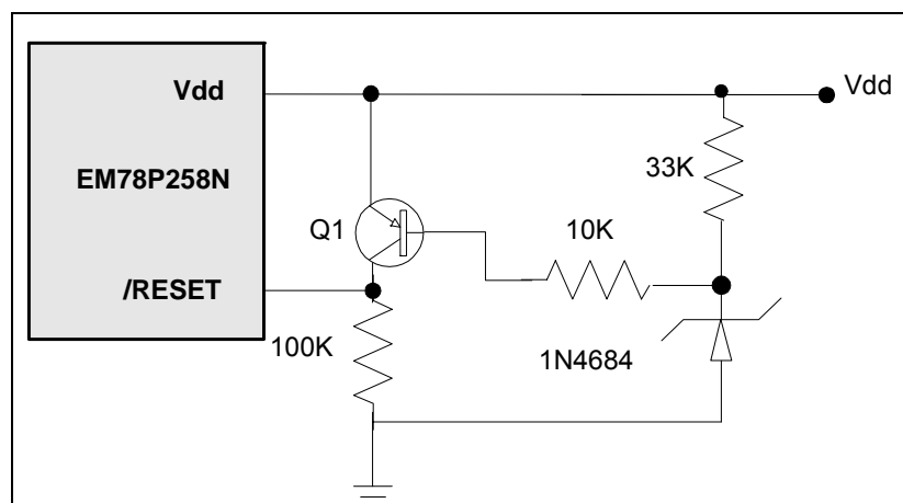
Fig 6-20 Residual Voltage Protection Circuit 1
