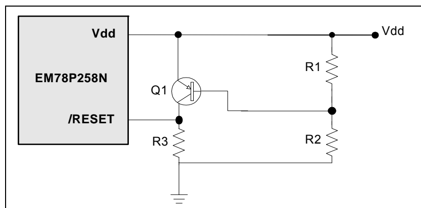
Fig 6-21 Residual Voltage Protection Circuit 2
