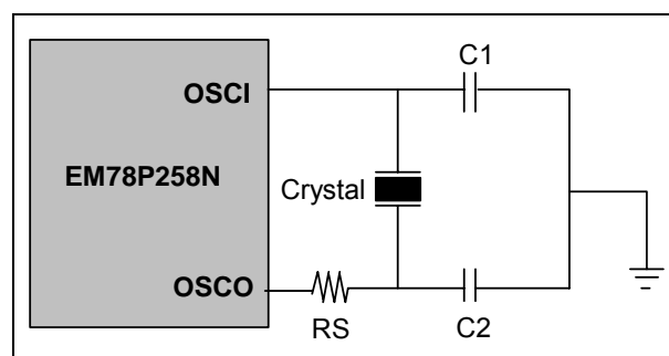
Fig 6-15 Crystal/Resonator Circuit
