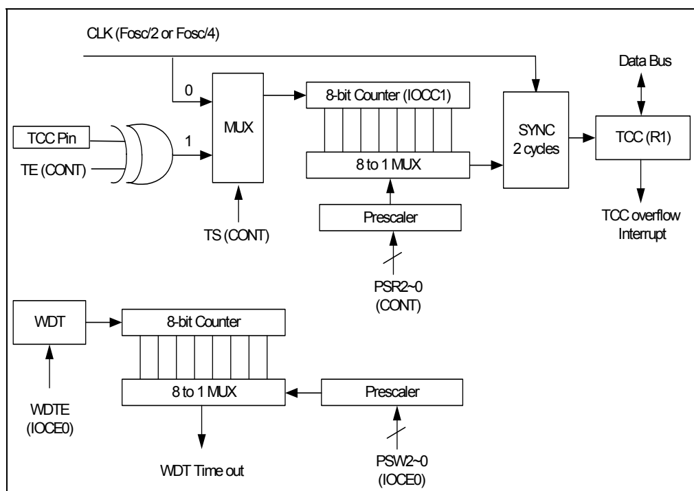
Fig 6-2 TCC and WDT Block Diagram
