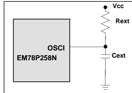
Fig 6-18 External RC Oscillator Mode Circuit
