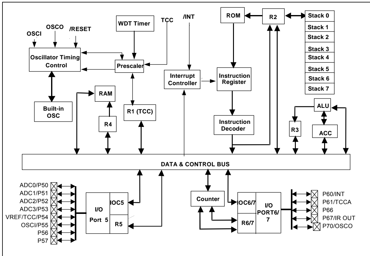
Fig 4-1 EM78P258N Functional Block Diagram
