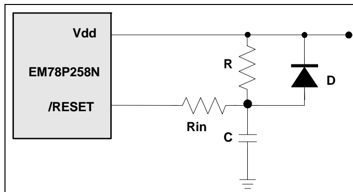
Fig 6-19 External Power on Reset Circuit
