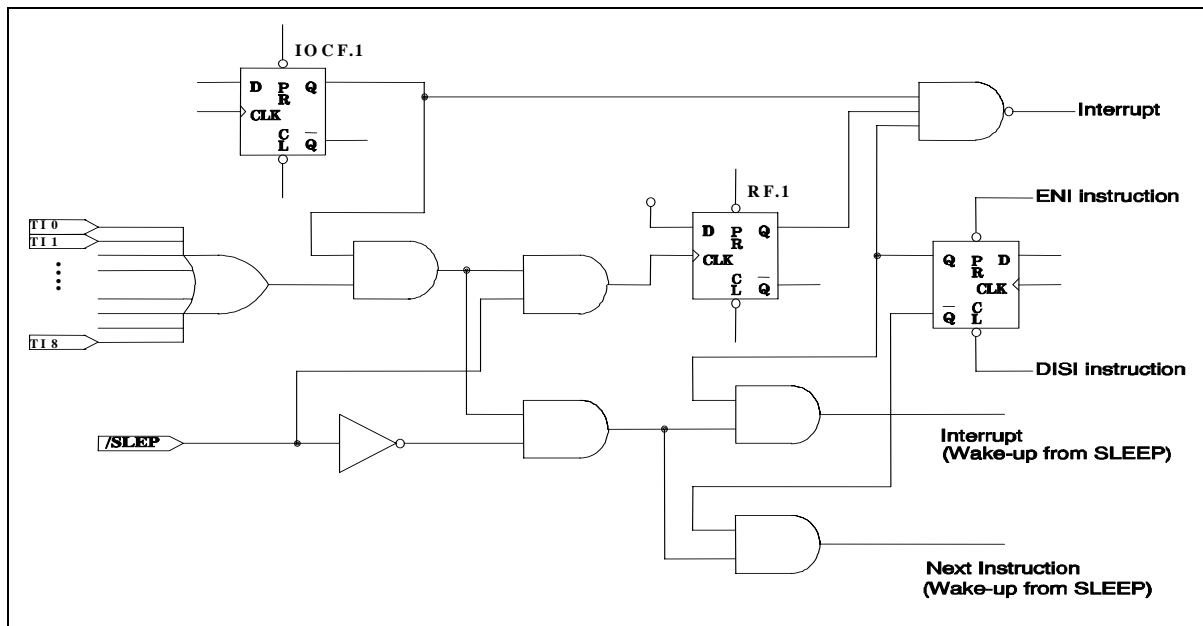
Fig 6-6 Port 5 Block Diagram with Input Change Interrupt/Wake-up
