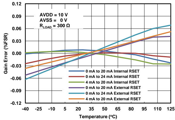
Figure 70. IOOUT Gain Error vs Temperature
