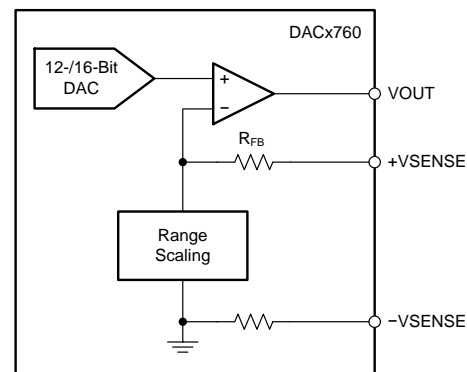
Figure 83. Voltage Output
