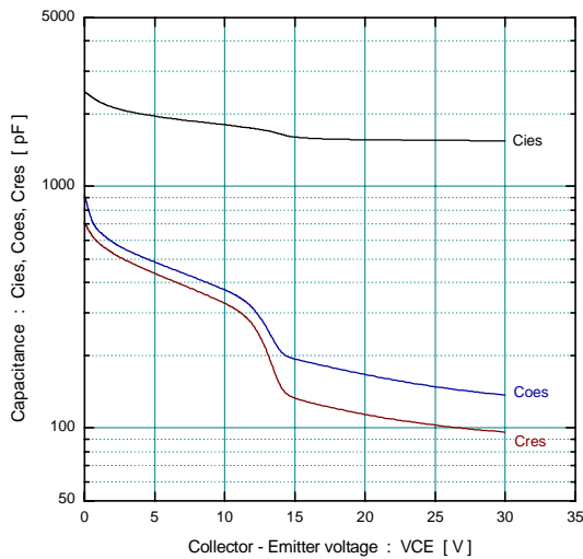
[ Brake ] Capacitance vs. Collector-Emittor voltage (typ.) V GE =0V, f= 1MHz, T j = 25°C
